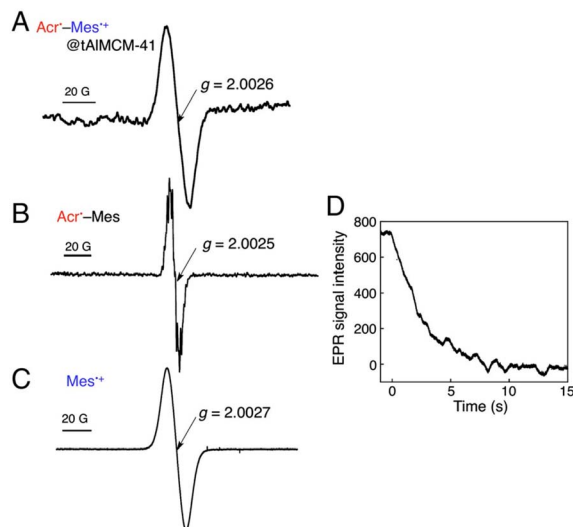
Fig. 5 (A) EPR spectrum of \text{Acr}^+-\text{Mes}^{*+} @tAlMCM-41 in MeCN at 298 K observed under photoirradiation ( \lambda > 390 nm) for 2 min. (B) EPR spectrum of \text{Acr}^+-\text{Mes} generated by the photoinduced ET reduction of \text{Acr}^+-\text{Mes} by BNAH (5.0 equiv.) in MeCN under photoirradiation. (C) EPR spectrum of mesitylene radical cation prepared by the photoinduced 1 e^- oxidation of mesitylene with \text{Hg}(\text{CF}_3\text{COO})_2 in \text{CF}_3\text{COOH} at 298 K under photoirradiation. (D) Decay time course of the EPR signal intensity due to \text{Acr}^+-\text{Mes}^{*+} @tAlMCM-41 in MeCN at 298 K. Reprinted with permission from ref. 67. Copyright 2012, National Academy of Sciences.
