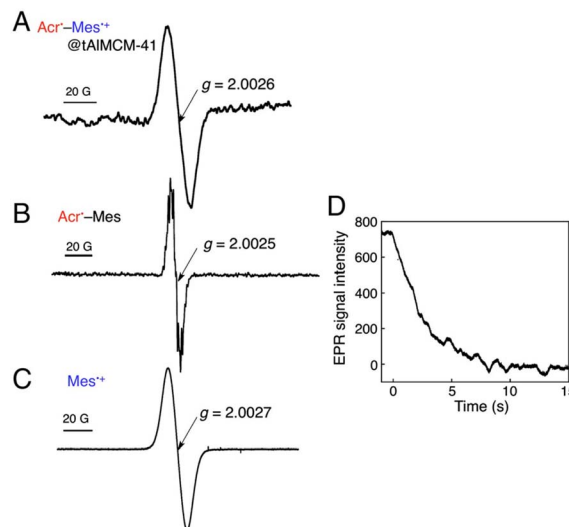
Fig. 5 (A) EPR spectrum of \text{Acr}^+-\text{Mes}^+ @tAIMCM-41 in MeCN at 298 K observed under photoirradiation ( \lambda > 390\text{ nm} ) for 2 min. (B) EPR spectrum of \text{Acr}^+-\text{Mes} generated by the photoinduced ET reduction of \text{Acr}^+-\text{Mes} by BNAH (5.0 equiv.) in MeCN under photoirradiation. (C) EPR spectrum of mesitylene radical cation prepared by the photoinduced 1\text{e}^- oxidation of mesitylene with \text{Hg}(\text{CF}_3\text{COO})_2 in \text{CF}_3\text{COOH} at 298 K under photoirradiation. (D) Decay time course of the EPR signal intensity due to \text{Acr}^+-\text{Mes}^+ @tAIMCM-41 in MeCN at 298 K. Reprinted with permission from ref. 67. Copyright 2012, National Academy of Sciences.
