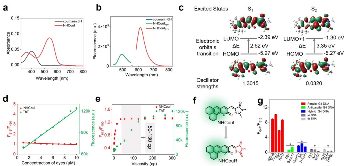
Fig. 3 (a) Absorption spectra of NHCou and NHCouI ( 5 \mu\text{M} ). (b) The emission spectra of NHCou and NHCouI ( 1 \mu\text{M} ) with NG16 ( 5 \mu\text{M} ). (c) The frontier orbital, energy gaps, and oscillator strengths of NHCouI in the S_1 and S_2 excited states are calculated by TDDFT at the B3LYP/6-31+g(d) level. (d) F_{613}/F_{490} ratio of NHCouI and fluorescence intensity of ThT as a function of the probe concentration ( 1 – 10 \mu\text{M} ) in response to NG16 ( 0.5 \mu\text{M} ). (e) The plot of the F_{613}/F_{490} ratio for NHCouI and the fluorescence intensity at 484 \text{ nm} for ThT as a function of viscosity, respectively. (f) Schematic diagram of the expanded molecular structure of NHCouR . (g) Fluorescence response of NHCouR ( 1 \mu\text{M} ) to different oligonucleotides ( 5 \mu\text{M} ). Data represent means \pm SD, n = 3 . P value was calculated based on the T -test ( *P < 0.05 ).
