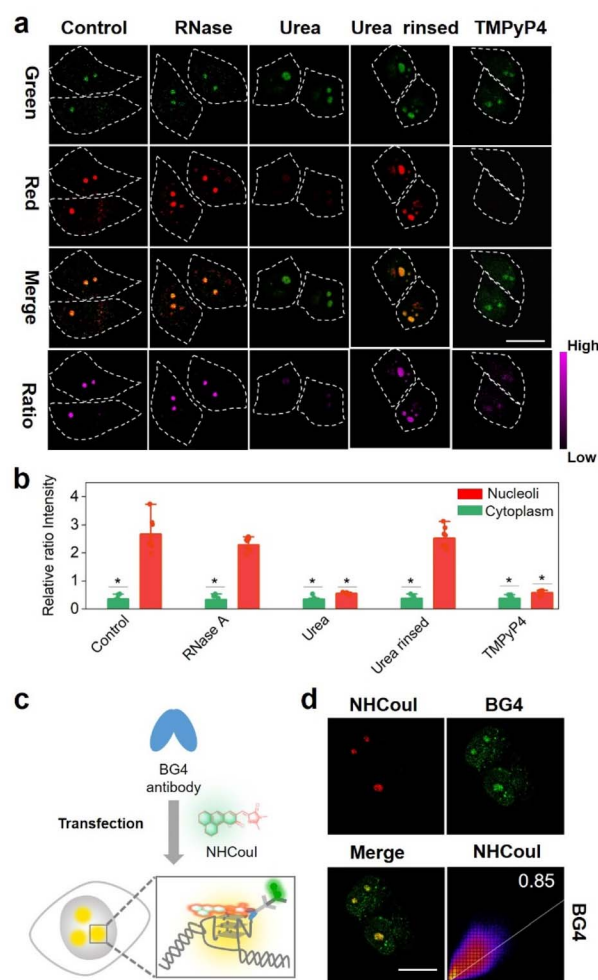
Fig. 4 (a) Two-channel ratiometric confocal imaging of fixed HeLa cells stained with NHCouI (5 \mu\text{M} ) before and after treatment of cells with RNase A, urea, rinsing to remove urea, and TMPyP4, respectively. "Ratio" represents red channel fluorescence divided by green channel fluorescence. (b) The quantification of the ratio of the fluorescence intensities of the nucleoli and cytoplasm in fixed HeLa cells processed by ImageJ. Data represent means \pm SD, n = 8 . P value was calculated based on T -test ( *P < 0.05 ). (c) Schematic illustration of the colocalization between NHCouI (red) and immunofluorescence staining of G4 structures by BG4 antibody (purple) in HeLa cells. (d) Immunofluorescence confocal microscopy image of fixed HeLa cells treated with the specific G-quadruplex antibody (BG4) and NHCouI (1 \mu\text{M} ). Excitation wavelength and emission filters: NHCouI : E_x/E_m : 405/500–550 nm; E_x/E_m : 561/570–620 nm. Alexa Fluor: 647: 640/663–738 nm. Scale bar = 20 \mu\text{m} .
