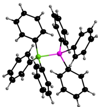
Fig. 10 Molecular structure of \text{Ph}_3\text{B}-\text{PPh}_3 1 . Thermal ellipsoids correspond to 25% probability except for the H atoms that are depicted with arbitrary radii; disorder is omitted for clarity.
