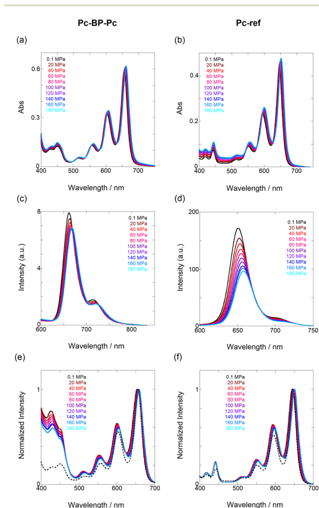
Fig. 2 (a–f) Pressure-dependent UV/vis spectra of (a) Pc-BP-Pc (82 \mu\text{M} ) and (b) Pc-ref (91 \mu\text{M} ); fluorescence spectra of (c) Pc-BP-Pc (79 \mu\text{M} ) ( \lambda_{\text{ex}} = 580 nm) and (d) Pc-ref (91 \mu\text{M} ) ( \lambda_{\text{ex}} = 543 nm); and excitation spectra of (e) Pc-BP-Pc (82 \mu\text{M} ) ( \lambda_{\text{em}} = 660 nm) and (f) Pc-ref (91 \mu\text{M} ) ( \lambda_{\text{em}} = 650 nm) in toluene at room temperature at 0.1, 20, 40, 60, 80, 100, 120, 140, 160, and 180 MPa (from black to sky blue), measured in a high-pressure cell. The black dotted lines represent the normalized UV/vis spectra at 0.1 MPa.
