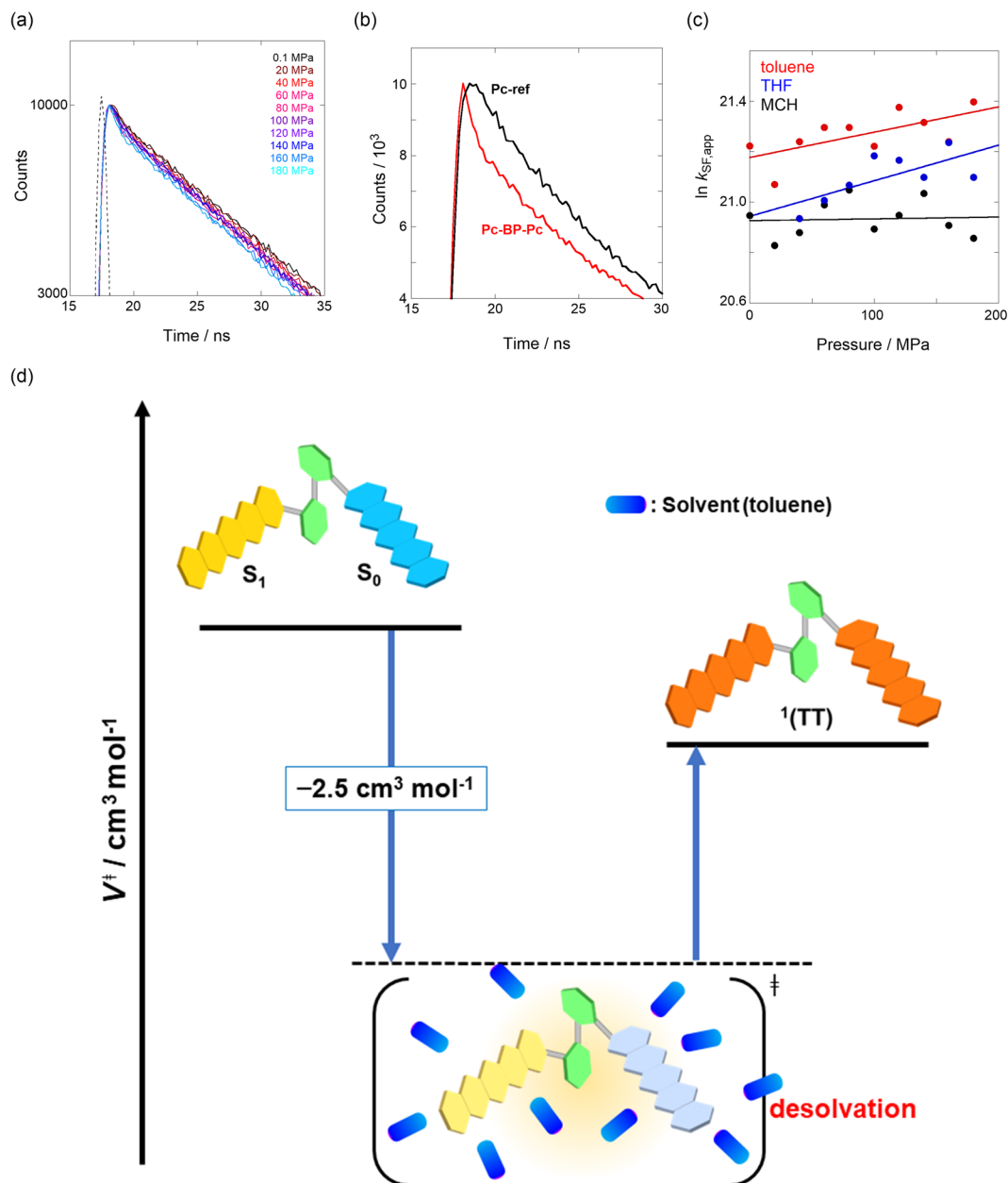
Fig. 3 (a and b) Enlarged time-correlated fluorescence decays ( \lambda_{\text{ex}} = 405 nm) of (a) Pc-BP-Pc (74 \mu\text{M} ) ( \lambda_{\text{em}} = 660 nm) in toluene at room temperature at 0.1, 20, 40, 60, 80, 100, 120, 140, 160, and 180 MPa (from black to sky blue) and (b) Pc-BP-Pc (74 \mu\text{M} ) ( \lambda_{\text{em}} = 660 nm, red) and Pc-ref. 89 \mu\text{M} ( \lambda_{\text{em}} = 650 nm, black) in toluene at room temperature at 180 MPa, measured in a high-pressure cell. The black dotted line represents the instrument response function. (c) Pressure dependence of SF rate constants ( k_{\text{SF,app}} ) of Pc-BP-Pc in toluene (red, correlation coefficient r = 0.655 ), THF (blue, r = 0.706 ), and MCH (black, r = 0.059 ) at room temperature; the separate plots with error bars are given in Fig. S26.† The large deviations for r are simply based on the roughness of the number of the digits in the lifetime apparatus. (d) Schematic diagram of Pc-BP-Pc for volumetric changes in the transition state via the intramolecular SF process.
