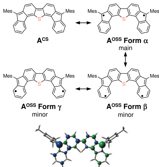
Fig. 3 Kekulé resonance structures of A CS and A OSS , as well as the optimized structure of A OSS showing the spin density. In the spin density plot, blue is positive and green is negative (isovalue: 0.005).
