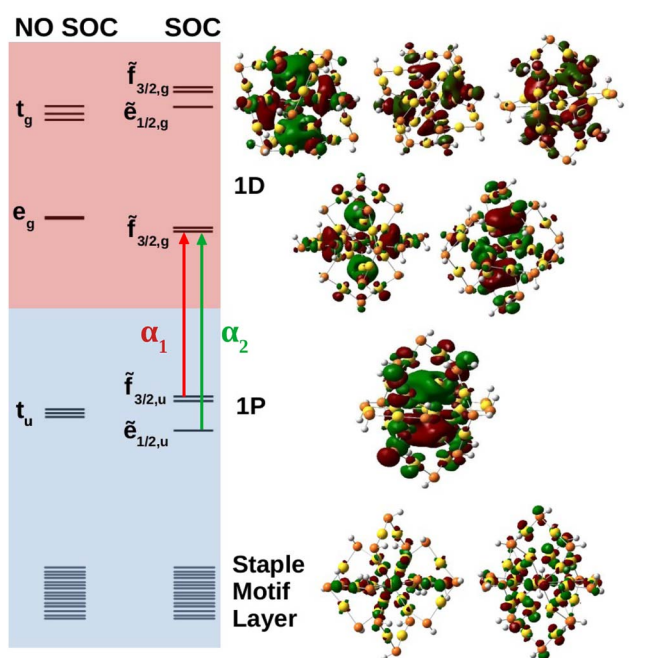
Fig. 4 MO diagram of Au_{25}(SH)_{18}^- with and without SOC, where each line is a Kramers pair. Blue and red shaded orbitals denote occupied and unoccupied orbitals, respectively. Below the superatomic orbitals exists a high density of states region where electron density is delocalized onto the staple motif layer. Images of the orbitals are shown on the right.
