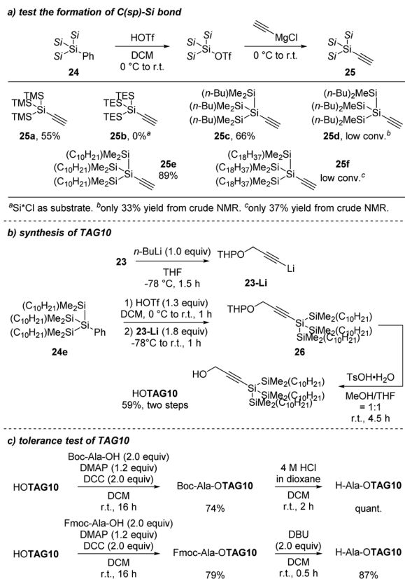
Scheme 13 Extension of the alkyl chains on the silicon atoms (a) test of the formation of C–Si bond; (b) synthesis of TAG10 ; (c) tolerance test of TAG10 .
