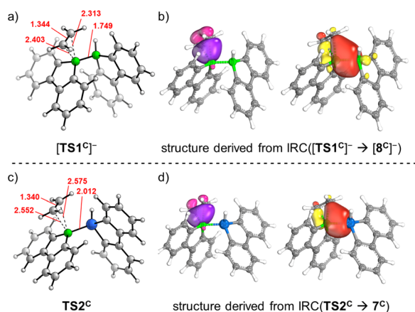
Fig. 2 (a) Computed geometry of [TS1^C]^\ddagger . (b) Two IBOs observed on a structure at 2.582 bohr amu 1/2 along the IRC( [TS1^C]^\ddagger \rightarrow [8^C]^- ) path; IBO contributions: left: C(dist) = 0.77, C(prox) = 0.76, prev. B(sp 2 ) = 0.43, others = 0.04; right: C(dist) = 0.08, C(prox) = 0.11, prev. B(sp 2 ) = 0.90, B(sp 3 ) = 0.74, others = 0.17. (c) Computed geometry of TS2^C . (d) Two IBOs observed on a structure at 15.076 bohr amu 1/2 along the IRC( TS2^C \rightarrow 7^C ) path; IBO contributions: left: C(dist) = 0.76, C(prox) = 0.65, prev. B(sp 2 ) = 0.55, others = 0.04; right: C(dist) = 0.10, C(prox) = 0.17, prev. B(sp 2 ) = 0.92, Si(sp 3 ) = 0.72, others = 0.08. Highlighted in red are selected bond lengths and atom...atom distances (in Å). Prox, dist: proximal, distal with respect to the B...E core; prev. = previously.
