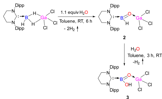
Scheme 3 Stepwise synthesis of -\text{hydrido} and -\text{hydroxy} oxoboranes, 2 and 3 from the reaction of 1 with water.
