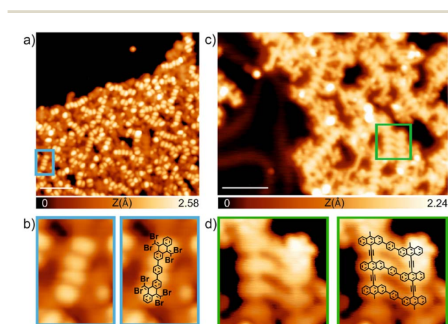
Fig. 8 On-surface deposition and reactivity of TBQ3 species on Au(111). (a) Overview STM image of the sublimation of a submonolayer coverage of TBQ3 on a pristine Au(111) surface kept at room temperature. V_b = 1 V, I_t = 100 pA, scale bar: 4.0 nm. (b) Left: Zoomed-in image of the blue rectangle indicated in panel (a) showing an intact molecule with two consecutive pairs of elongated bright protrusions. Right: Superposition of the chemical model. (c) Long-range STM image after the annealing of (a) at 150 °C. V_b = 0.5 V, I_t = 50 pA, scale bar: 4 nm. (d) Left: Zoomed-in image of the green highlighted area in panel (c). Right: Superposition of the chemical model.
