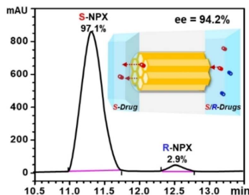
Fig. 29 Schematic representation of chiral COF-packed nanochannel membrane to solve the challenge of enantioselectivity and HPLC chromatogram of separated naproxen through the L-Tyr-COF channel membrane. 76 Reproduced with permission from ref. 76. Copyright 2022, John Wiley and Sons.
