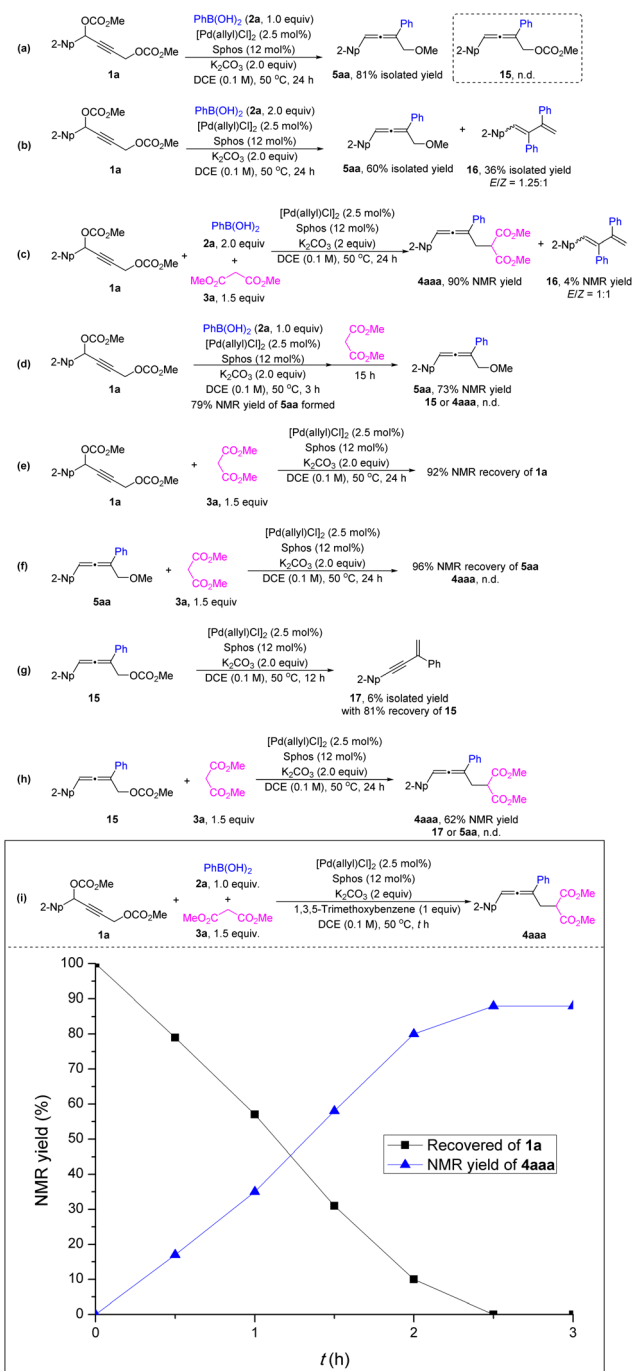
Scheme 3 Mechanistic studies.
