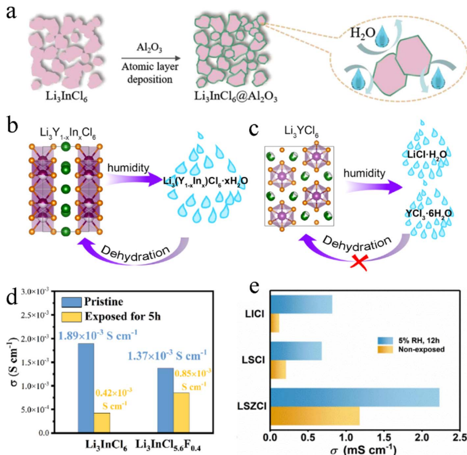
Fig. 15 (a) Schematic diagram showing that the Al_2O_3 coating enhanced Li_3InCl_6 air stability via powder atomic layer deposition. Reproduced with permission. 158 Copyright 2021, Wiley-VCH. Schematic illustration of the humidity stabilities of (b) Li_3Y_{1-x}In_xCl_6 and (c) Li_3YCl_6 , respectively. Reproduced with permission. 38 Copyright 2020, American Chemical Society. (d) Ionic conductivity evolution of Li_3InCl_6 and Li_3InCl_{5.6}F_{0.4} after being exposed to a dew-point dry room ( -20 \pm 3\ ^\circ C ) for 5 h. Reproduced with permission. 115 Copyright 2022, Elsevier B.V. (e) Ionic conductivity of Li_3InCl_6 , Li_3ScCl_6 , and Li_{2.5}Sc_{0.5}Zr_{0.5}Cl_6 before and after exposure to an Ar atmosphere with 5% relative humidity. Reproduced with permission. 115 Copyright 2022, Elsevier B.V.
