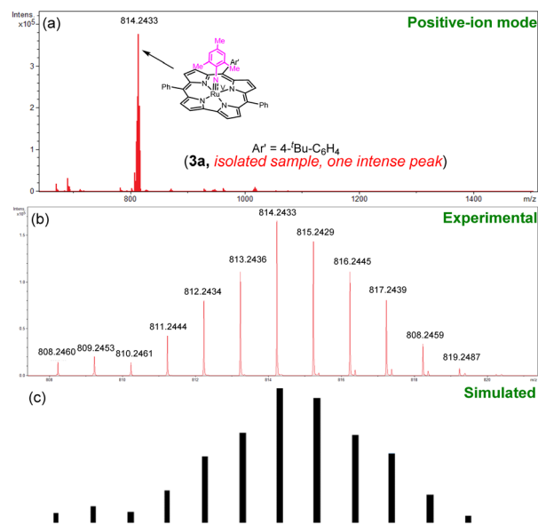
Fig. 2 (a) HR-ESI-MS (positive-ion mode) spectrum of [\text{Ru}^{\text{V}}(\text{Bu-Cor})(\text{NMes})] ( 3a ). (b) Experimental isotope pattern of [\text{Ru}^{\text{V}}(\text{Bu-Cor})(^{14}\text{NMes})]^+ + [\text{Ru}^{\text{V}}(\text{Bu-Cor})(^{15}\text{NMes})]^+ in a 1:1 ratio (50% ^{15}\text{N} enrichment). (c) Simulated pattern of (b).
