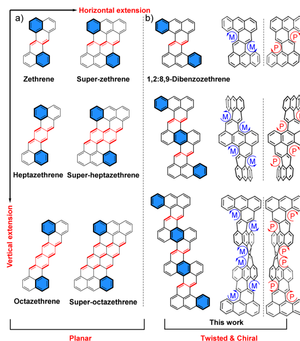
Fig. 1 (a) Zethrene and horizontally and vertically extended zethrenes; (b) 1,2:8,9-dibenzozethrene (DBZ) and vertically fused DBZ oligomers reported in this work and their representative enantiomers.
