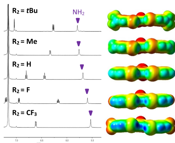
Fig. 3 1 H NMR spectra (C 6 D 6 , 500 MHz, 5 mM) of 2R 2 -G3XB derivatives (left) highlighting the HBeXB downfield shift of the amine as the halogen becomes more electron rich; ESP maps (isovalue = 0.001 a.u.) for 2R 2 -G3XB derivatives (right) are displayed on the same scale. Electron deficient regions are blue and electron rich regions are red.
