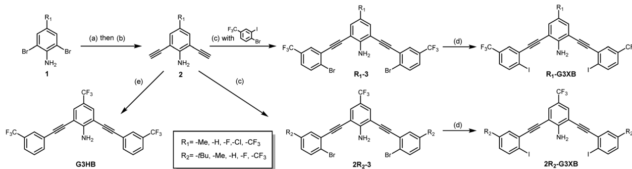
Scheme 1 Synthesis of G3XB derivatives and controls used to study HBeXB substituent effects. Reagents and conditions: (a) TMS-acetylene, Pd(PPh 3 ) 2 Cl 2 , Cu(I)I, DIPEA, DMF, overnight, N 2 , 80 °C; (b) K 2 CO 3 , MeOH/DCM (1 : 1 v/v), 4 hours, rt, 45–96%; (c) 4-Bromo-3-iodo-R 2 -benzene, Pd(PPh 3 ) 2 Cl 2 , Cu(I)I, DIPEA, DMF, overnight, N 2 , rt, 53–87%; (d) NaI, Cu(I)I, trans -N,N-dimethylcyclohexane-1,2-diamine, 1,4-dioxane, microwave reactor, 12–24 hours, 150 °C, 33–84%; (e) 3-bromotrifluoromethylbenzene, Pd(PPh 3 ) 2 Cl 2 , Cu(I)I, DIPEA, DMF, overnight, N 2 , 80 °C, 60%.
