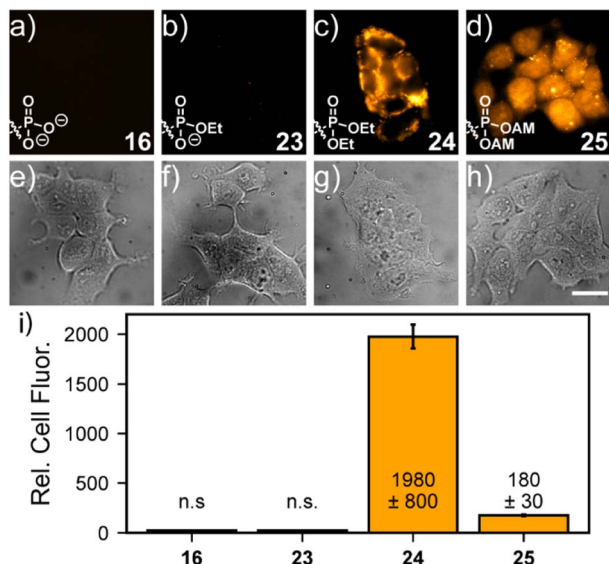
Fig. 2 Tunable localization of 3-phosphonoTMRs. Widefield fluorescence (a–d) and transmitted light (e–h) images of HEK293T cells stained with 500 nM dyes 16 (a and e), 23 (b and f), 24 (c and g), or 25 (d and h) in HBSS for 20 min at 37 °C. Quantification (i) of cellular fluorescence. Values are mean fluorescence intensity ± S.E.M. for n = 21 , 32, 45, and 19 regions of interest (ROI) for each dye. Each ROI contained between 2 and 20 individual cells. “n.s.” means that the cellular fluorescence values were not above background fluorescence. Coverslips were placed into fresh HBSS prior to imaging. Scale bar is 20 \mu\text{m} .
