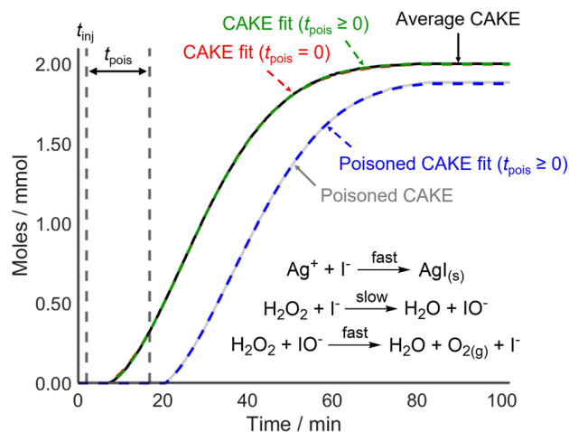
Fig. 5 CAKE plot of gaseous \text{O}_2 evolution over time for \text{I}^- -catalyzed \text{H}_2\text{O}_2 decomposition as measured using displacement, in the absence (black, see Fig. 2) and presence (grey) of \text{Ag}^+ poison. Different CAKE fits were obtained when disallowing poisoning (dashed red, see Fig. 2) or allowing poisoning (dashed green and dashed blue, respectively). Allowing for poisoning, fitted parameters in the absence of \text{Ag}^+ : k = 5.7 \pm 0.2 \times 10^{-3} \text{ M}^{-0.82} \text{ s}^{-1} , m = 0.985 \pm 0.004 , n = 0.835 \pm 0.008 , t_{\text{pois}} = 3.47 \pm 0.07 min, catalyst poisoning = 0.069 \pm 0.001 mmol. Fitted parameters in the presence of \text{Ag}^+ : k = 4.2 \pm 0.2 \times 10^{-3} \text{ M}^{-0.69} \text{ s}^{-1} , m = 0.908 \pm 0.006 , n = 0.78 \pm 0.02 , t_{\text{pois}} = 14.9 \pm 0.2 min, catalyst poisoning = 0.298 \pm 0.004 mmol.
