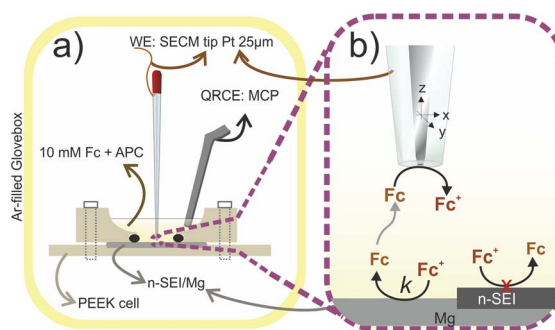
Scheme 1 (a) Illustration of the SECM electrochemical cell with a Pt microelectrode ( 12 \mu\text{m} tip radius) used as the working electrode (WE). A Chevrel phase (MCP) electrode was used as the quasi-reference counter electrode (QRCE) for the n-SEI evaluation. The FB-SECM compartment was filled with APC electrolyte containing 10 mM Fc. (b) Scheme of the FB-SECM mode to interrogate the rate of the electron transfer reaction at the sample surface. All measurements were performed inside an Ar-filled glovebox.
