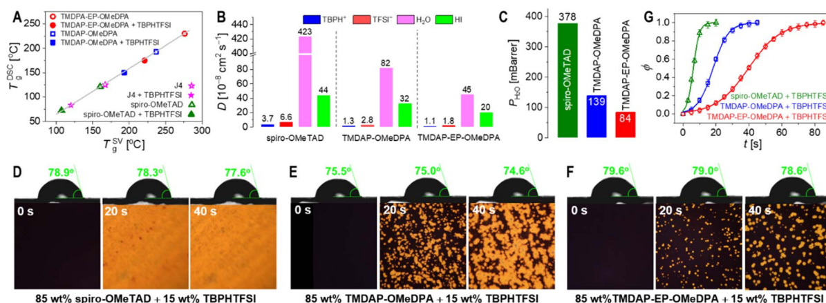
Fig. 4 (A) Correlation between glass transition temperatures obtained from molecular dynamics simulation ( T_g^{\text{SV}} ) and differential scanning calorimetry measurement ( T_g^{\text{DSC}} ). The weight percentage of TBPHTFSI is 15%. (B) 80 °C diffusivity ( D ) for internal and external species in an organic semiconductor composite containing 15 wt% TBPHTFSI. (C) Water permeability ( P_{\text{H}_2\text{O}} ) obtained from molecular dynamics simulation for the 15 wt% TBPHTFSI-containing organic semiconductor composite. (D–F) Evolution of water contact angle (values in green) and polarized optical microscope images over time for a perovskite film covered with a hole transport layer under a water droplet. The hole transport layer composition is also provided. The polarized optical microscope image size is 500 × 500 \mu\text{m} . (G) Time-dependent percentage ( \phi ) of the yellow region in polarized optical microscope images.
