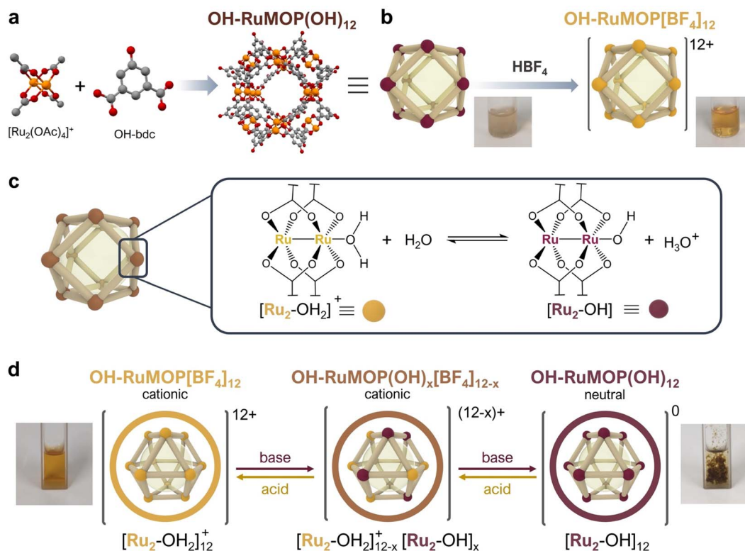
Fig. 1 (a) Schematic representation of the synthesis of \text{OH-RuMOP}(\text{OH})_{12} from its building blocks. (b) Transformation of non-soluble \text{OH-RuMOP}(\text{OH})_{12} into soluble \text{OH-RuMOP}[\text{BF}_4]_{12} due to the removal of coordinated \text{OH}^- ligands upon acid treatment with \text{HBF}_4 . (c) Acid–base equilibrium between water-coordinated and hydroxo-coordinated \text{Ru}_2(\text{CO}_2)_4 paddlewheel units in water solutions. (d) Schematic representation of the gradual interconversion between cationic \text{OH-RuMOP}[\text{BF}_4]_{12} and neutral \text{OH-RuMOP}(\text{OH})_{12} upon acid/base treatment.
