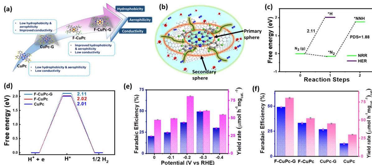
Fig. 5 (a) Scheme representing the limitations and improvements of different catalysts, (b) scheme showing the mechanistic pathway of \text{N}_2 diffusion through primary and secondary spheres in F-CuPc-G, (c) free energy profile of \text{N}_2 and NNH adsorption on F-CuPc-G, (d) free energy profile of the HER for F-CuPc-G, F-CuPc and CuPc systems. The bar plot diagrams illustrating the FE and yield rate (e) at different potentials for F-CuPc-G, and (d) for different catalysts.
