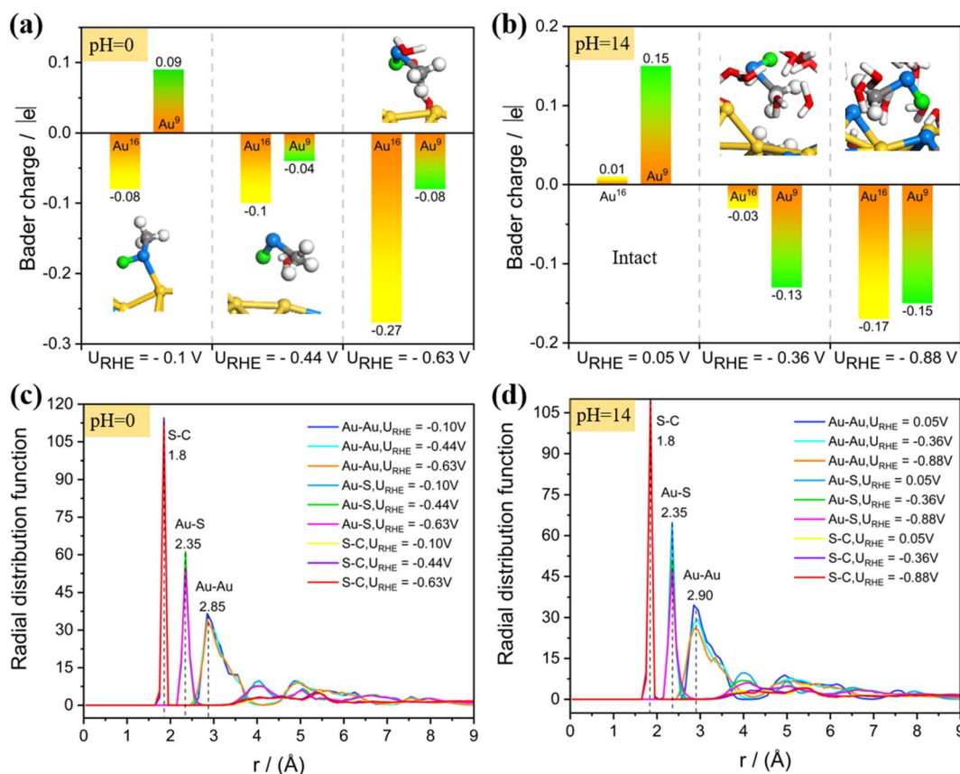
Fig. 5 Evolution of Bader charge on the under-coordinated bare Au atoms from de-thiolated \text{Au}_{25} NC at different potentials after AIMD simulations for the acid (a) and alkaline system (b). Radial distribution function (RDF) of Au-Au, Au-S and S-C bonds from the equilibrated AIMD trajectory in (c) acid and (d) alkaline systems.
