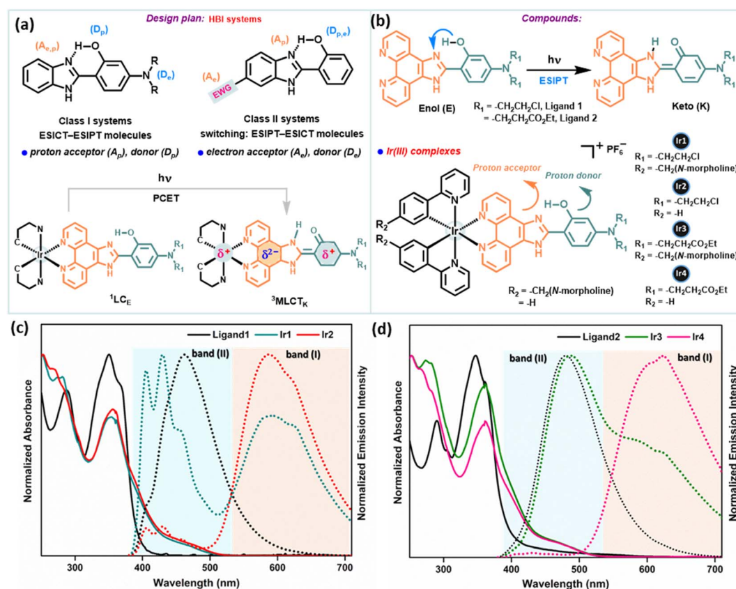
Fig. 2 (a) Design plan for synthesizing desired compounds. (b) Structures of phenanthroline-BIP based ancillary ligands attributing to the ESIP-ESICT phenomenon and the corresponding Ir(III)-complexes. The proton-accepting and donating parts are indicated in orange and cyan dark colors, respectively. (c) and (d) Normalized UV-vis absorption spectra (solid line) and the corresponding emission spectra (dotted line) of (c) ligand1, Ir1 and Ir2; (d) ligand2, Ir3 and Ir4; in DCM (10 \mu M), respectively under 365 nm excitation. Two emission bands are assigned as major band (I) and minor band (II), respectively.
