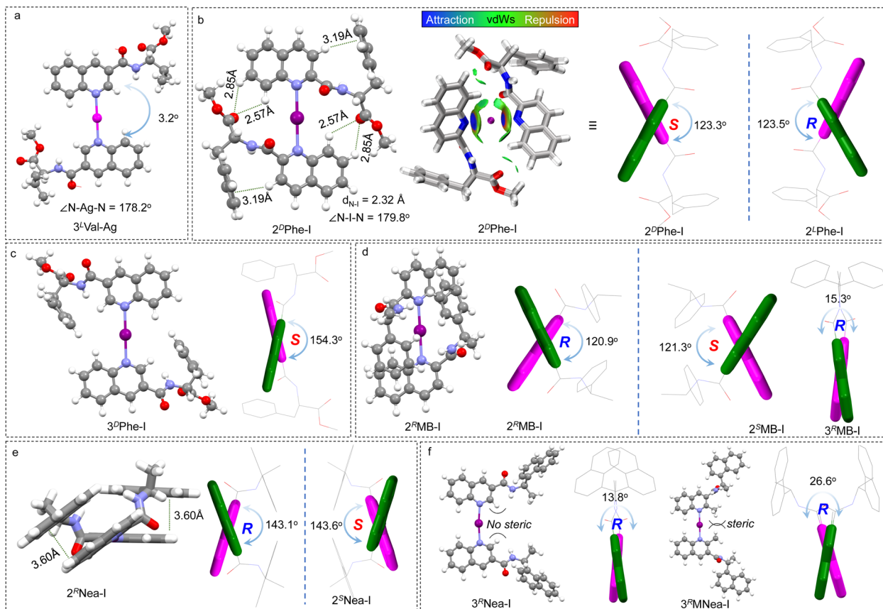
Fig. 2 (a) X-ray crystal structure of the 3 1 -Val-Ag complex. (b–f) DFT-optimized geometries of different halogen-bonded complexes. The R and S stand for the intrinsic axial chirality of biquinoline. Inset of (b) shows the IGMH analysis of 2 D Phe-I (isosurface = 0.008 a.u.). For clarity, quinoline moieties are displayed in green and purple colors.
