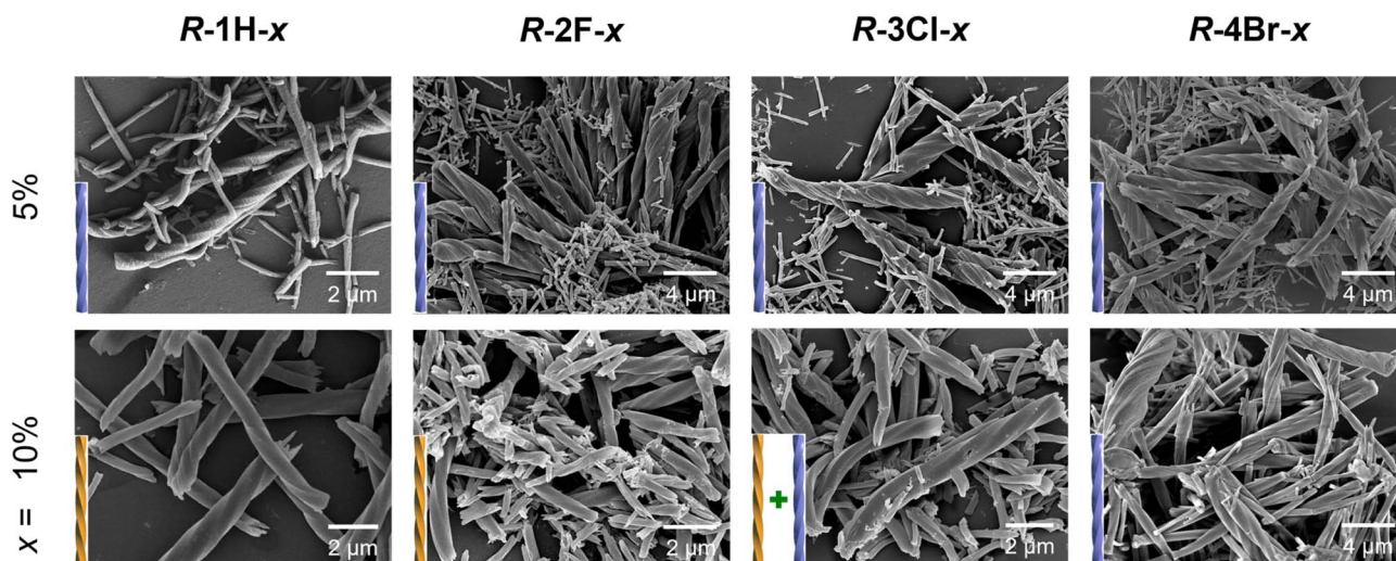
Fig. 6 SEM images of R\text{-1H-x} , R\text{-2F-x} , R\text{-3Cl-x} , and R\text{-4Br-x} with different x values ( 5\% and 10\% ) which are obtained at \text{pH } 5.0 and 100\text{ }^\circ\text{C} .
