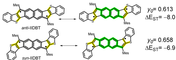
Scheme 4 Diradical forms contributing to the stabilization of anti - and syn -indenodibenzothiophes ( anti -IIDBT and syn -IIDBT). y_0 and experimental SQUID \Delta E_{ST} in kcal mol -1 are shown.
