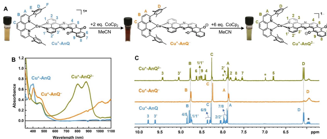
Fig. 4 (A) Reduction of Cu + -AnQ. (B) UV-vis spectra of Cu + -AnQ treated with CoCp 2 in CH 3 CN. (C) 1 H NMR of the reduced species generated by CoCp 2 . (Solvent: CD 3 CN; impurity is denoted by asterisk).
