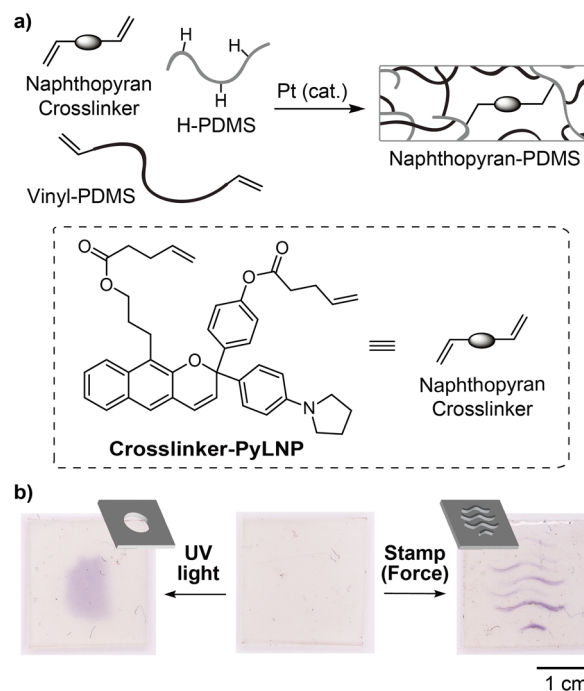
Fig. 3 (a) PDMS networks covalently crosslinked with linear 2H -naphthopyran mechanophore Crosslinker-PyLNP ( 1.5 \text{ wt\%} ) prepared via Pt-catalyzed hydrosilylation. (b) Photographs of the material before and after photoirradiation with 365 \text{ nm} UV light for 120 \text{ s} through a photomask, and after mechanical force applied via compression ( 2\times ) using an embossed stamp. Schematic representations of the photomask and stamp are shown.
