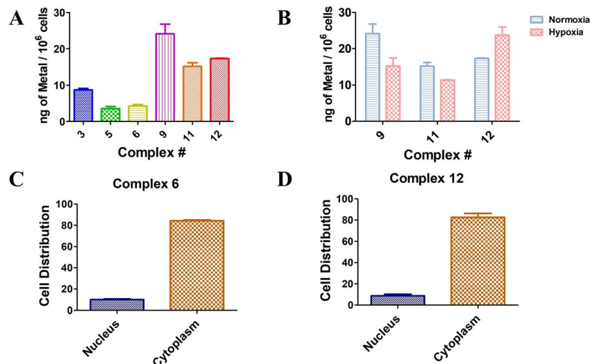
Fig. 5 (A) Cellular uptake of Ru(II) complexes 3, 5, and 6 and Os(II) complexes 9, 11, and 12 (5 μM and 4 h) in A549 cells determined by ICP-MS; (B) cellular uptake of Os(II) complexes 9, 11, and 12 (5 μM and 4 h) in A549 cells determined by ICP-MS under normoxic conditions and hypoxic conditions; (C) cellular fraction of complex 6 in different parts of A549 cells; (D) cellular fraction of complex 12 in different parts of A549 cells. All the experiments were performed in triplicate.
