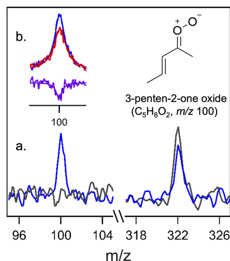
Fig. 1 (a) Mass spectra recorded with 118 nm photoionization of the (Z)-2,4-diiodopent-2-ene precursor (gray). Upon photolysis of the precursor at 248 nm in a 20% O 2 /Ar carrier gas, the m/z 322 mass peak arising from the precursor (C 5 H 8 I 2 ) is decreased and a new mass peak appears at m/z 100 with C 5 H 8 O 2 composition (blue), which is ascribed to the 3-penten-2-one oxide CI. (b) The m/z 100 photoionization signal (blue) decreases upon 410 nm ( ca. 4 mJ per pulse) excitation (red) with the difference trace (violet) illustrating the depletion signal. Also shown is the lowest energy tEE conformer of 3-penten-2-one oxide.
