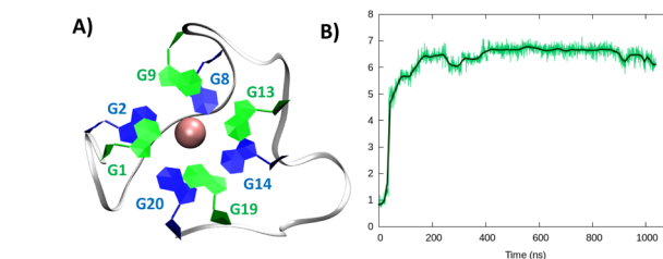
Fig. 3 A representative snapshot of the hybrid G4 formed by the RG-2 sequence as obtained by MD simulations. Guanine residues composing the two superposing tetrads are evidenced by different colours (A). The corresponding time series of the RMSD for the RNA strand (B). Analogous results obtained for the second replica are reported in Fig. S3B.†
