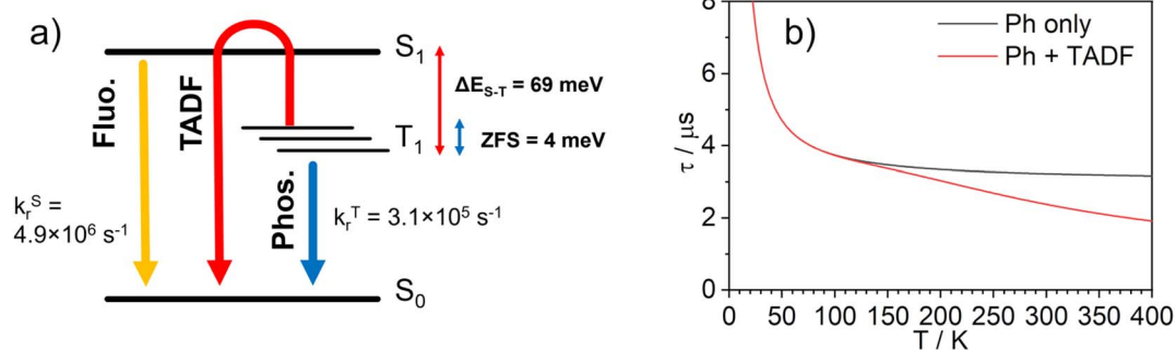
Fig. 7 (a) Computational model of the photophysics of 1 ; (b) simulated natural lifetime, \tau_0 , of 1 as a function of temperature obtained using eqn (3). The grey line represents the lifetime simulated without inclusion of a TADF component ( i.e. , phosphorescence only, k_r^S = 0 or \Delta E_{\text{ST}} = \infty ), and the red line the corresponding simulation in which the TADF component to the decay is included.
