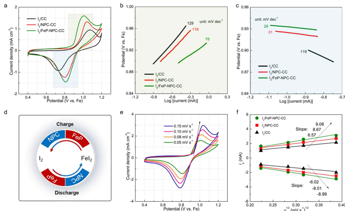
Fig. 5 Kinetic analyses of bidirectional catalysis-facilitated iodine redox. (a) CV profiles of Fe-I_2 coin cells assembled with different cathodes at a scan rate of 0.05 mV s^{-1} . Tafel plots calculated from the peaks of (b) iodine oxidation and (c) reduction in (a). (d) Schematic diagram of the bidirectional catalysis-directed iodine redox reactions during battery cycling. (e) CV curves of I_2/FeP-NPC-CC cathode at various scan rates. (f) Linear fitting of anodic and cathodic peaks versus square root of scan rate for different electrodes as noted.
