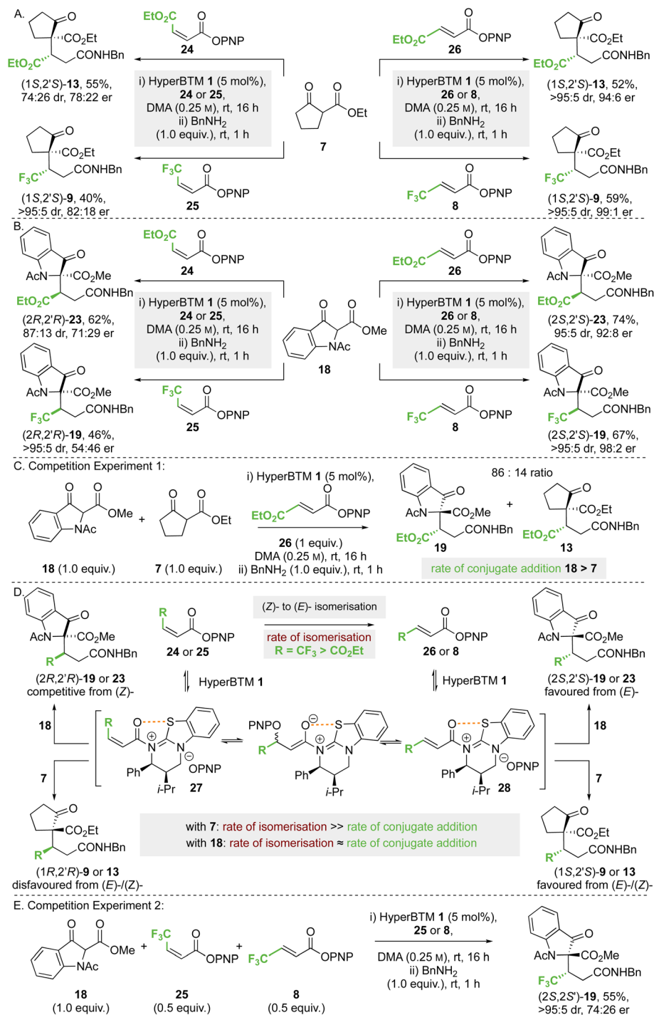
Scheme 6 Effect of ( Z - or E -) enoate configuration on stereoselectivity. All ers determined by HPLC analysis on a chiral stationary phase. All product drs determined by 1 H NMR analysis of the crude reaction mixture. Yields are isolated yields after purification.
