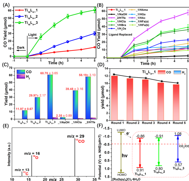
Fig. 7 (A) Time-dependent CO generation profiles for \text{Ti}_{16}\text{L}_4\text{-1/2/3} ; (B) time-dependent CO generation profiles for \text{Ti}_{16}\text{L}_4 with various ligand modifications; (C) CO production rates over \text{Ti}_{16}\text{L}_4 ; (D) durability assessments of \text{Ti}_{16}\text{L}_4\text{-1} . (E) ^{13}\text{C} recorded under ^{13}\text{CO}_2 atmosphere; (F) the energy band structure diagram for \text{Ti}_{16}\text{L}_4 . Reaction conditions: 3 mg of \text{Ti}_{16}\text{L}_4 , 10 mg [\text{Ru}(\text{bpy})_3]\text{Cl}_2 \cdot 6\text{H}_2\text{O} , 5 mL triethanolamine (TEOA), acetonitrile (8 mL), \text{H}_2\text{O} (2 mL), \text{CO}_2 (1 atm), \lambda \geq 420 nm, 25 °C, 5 h.
