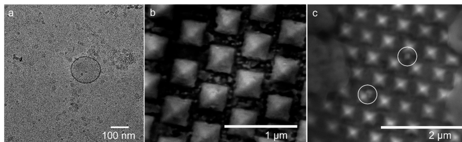
Fig. 2 a) Cryo-EM image of sEVs; b) SEM image of the SERS gold nanopyramid substrate; c) SEM image of the SERS gold nanopyramid substrate after sample introduction.
