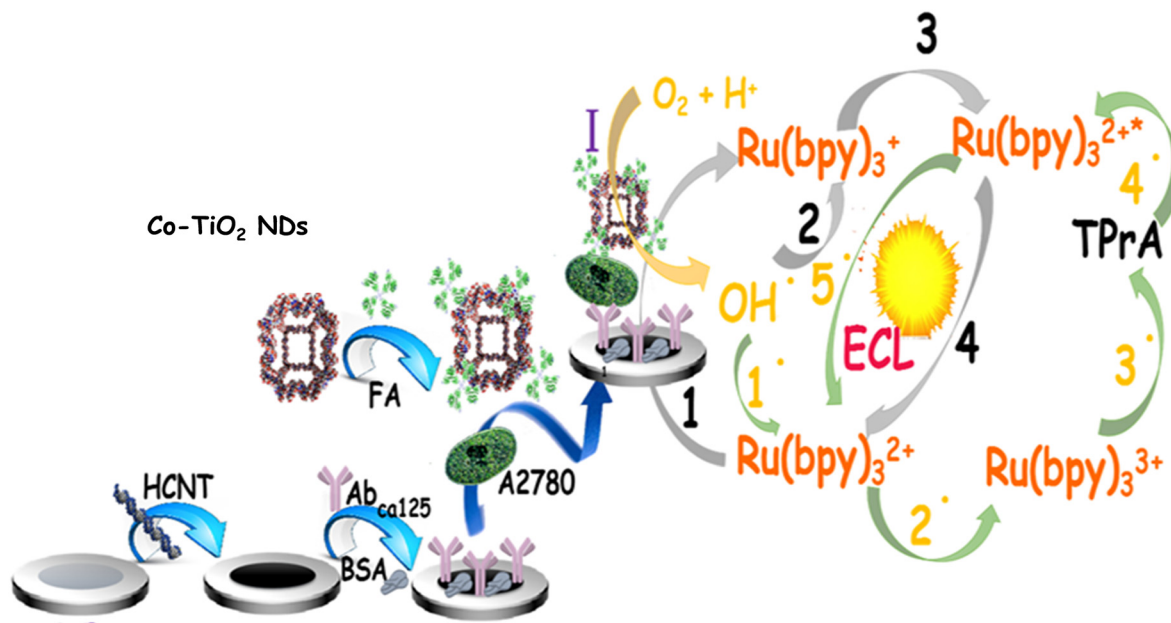
Scheme 1 The fabrication process of this biosensor.
