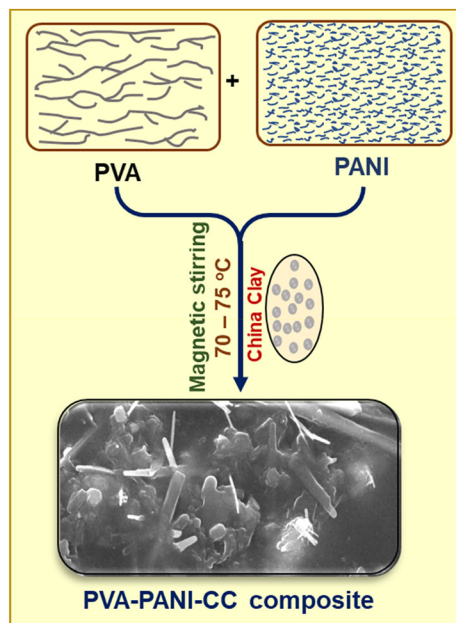
Fig. 1 Experimental setup for the preparation of PVA-PANI-CC.
