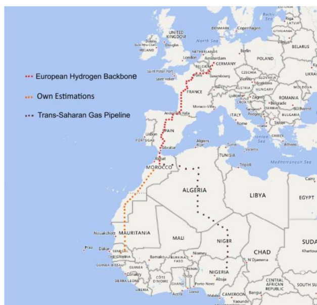
Fig. 1 Hydrogen supply chain. Red-colored route is possible corridor for German imports based on existing natural gas infrastructure (European Hydrogen Backbone). 28 The routes in Africa are estimated on the basis of our own calculations and the planned Trans-Saharan Gas Pipeline project.
