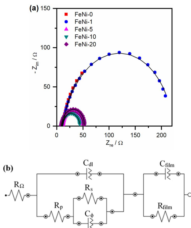
Fig. 6 (a) Nyquist plots for pristine and iron-incorporated nickel hydroxide films measured at 1.52 \text{ V} vs. RHE in an alkaline medium ( 1.0 \text{ M NaOH} ) and (b) equivalent circuit employed for fitting the Nyquist plots.
