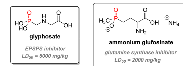
Fig. 21 Common organophosphorus herbicides.
