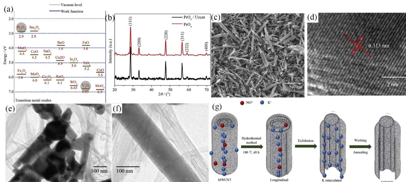
Fig. 17 Summary of oxide work functions and structural characterization of samples: (a) summary of the work functions of different oxides, (b) XRD of \text{PrO}_x and \text{PrO}_x/\text{U}_{\text{zcat}} samples, (c) SEM images of \text{PrO}_x/\text{U}_{\text{zcat}} , (d) HR-TEM images of \text{PrO}_x/\text{U}_{\text{zcat}} , (e and f) TEM images of \text{PrO}_x/\text{U}_{\text{zcat}} , (g) schematic illustration of the formation of zipping carbon nanotubes.
