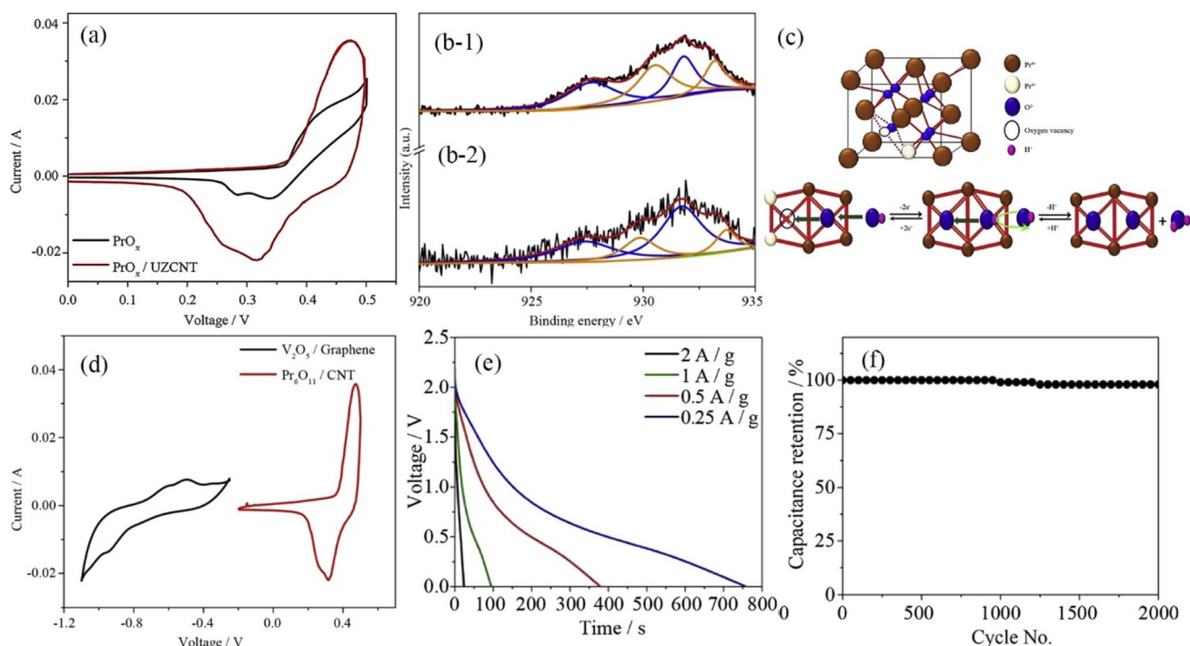
Fig. 18 XPS and electrochemical properties of \text{PrO}_x and \text{PrO}_x/\text{U}_{\text{zcat}} : (a) CV curves of \text{PrO}_x and \text{PrO}_x/\text{U}_{\text{zcat}} at 50 \text{ mV s}^{-1} , (b-1) XPS spectra of the Pr 3d state before charging, (b-2) XPS spectra of the Pr 3d state after charging, (c) formation mechanism of oxygen vacancies, (d) CV curves of \text{Pr}_6\text{O}_{11}/\text{CNT} and \text{V}_2\text{O}_5/\text{graphene} at 50 \text{ mV s}^{-1} , (e) the charge-discharge curve of the asymmetric capacitor after 2000 cycles, (f) cyclic stability of the asymmetric capacitor.
