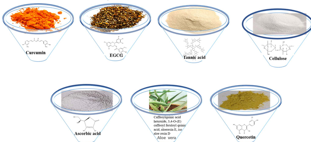
Fig. 2 Phytochemicals: source, occurrence and chemical structure.
