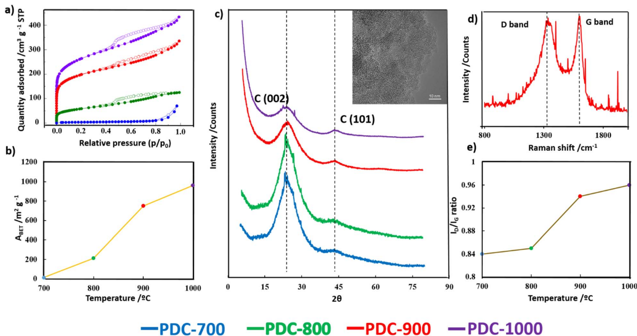
Fig. 2 (a) \text{N}_2 adsorption (full symbols) – desorption (empty symbols) isotherms of the PDC- T series; (b) plot of A_{\text{BET}} obtained from \text{N}_2 adsorption isotherms; (c) XRD patterns of the PDC- T series and TEM image of PDC-900 (inset); (d) Raman spectra of PDC-900; and (e) plot of I_{\text{D}}/I_{\text{G}} ratio obtained from Raman spectra.
