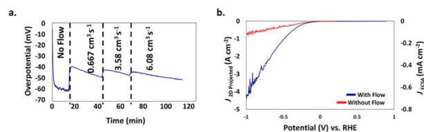
Fig. 7 (a) Impact of flow rate on the overpotential of the 3D printed NiMo flow-through electrode for HER at J_{2\text{D,projected}} = 10 mA \text{cm}^{-2} as a function of time. (b) J_{2\text{D,projected}} (left axis) and J_{3\text{D,ECSA}} (right axis) of the potential vs. RHE in a traditional electrode configuration (red) and in a flow-through configuration at a flow rate of 3.58 \text{cm}^3 \text{s}^{-1} (blue) [reproduced from ref. 29, with kind permission].
