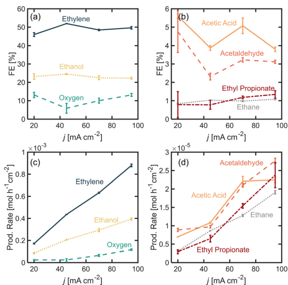
Fig. 3 Faradaic efficiency (FE) for the different propionic acid oxidation (a) major and (b) minor products, as well as oxygen as a function current density j , for [\text{PA}]_0 = 2 \text{ M} . Production rate for the different propionic acid oxidation (c) major and (d) minor products, as well as oxygen as a function current density j . Electrolyte \text{pH}_0 was 7 \pm 0.2 . The reaction volume was 14 mL. Experiments performed in a divided H-cell, using Nafion® as a proton exchange. Electrolyte was \text{Na}_3\text{PO}_4 0.5 M and the initial electrolyte mixture was kept at room temperature. The reaction time of each experiment was selected to maintain the total charge transferred constant for the different current densities, and they were 116, 52, 34 and 25 min for j = 20, 45, 70, 95 \text{ mA cm}^{-2} respectively. A cold trap was implemented downstream of the gas effluent to condense any liquid products evaporated during the reaction.
