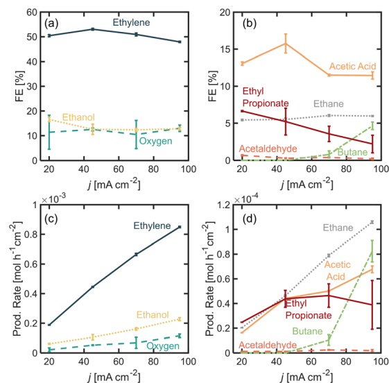
Fig. 4 Faradaic efficiency (FE) for the different propionic acid oxidation (a) major and (b) minor products, as well as oxygen as a function current density j , for [\text{PA}]_0 = 6 \text{ M} . Production rate for the different propionic acid oxidation (c) major and (d) minor products, as well as oxygen as a function current density j . Electrolyte \text{pH}_0 was 7 \pm 0.2 . The reaction volume was 14 mL. Experiments performed in a divided H-cell, using Nafion® as a proton exchange. Electrolyte was \text{Na}_3\text{PO}_4 0.5 M and the initial electrolyte mixture was kept at room temperature. The reaction time of each experiment was selected to maintain the total charge transferred constant for the different current densities, and they were 116, 52, 34 and 25 min for j = 20, 45, 70, 95 \text{ mA cm}^{-2} respectively. A cold trap was implemented downstream of the gas effluent to condense any liquid products evaporated during the reaction.
