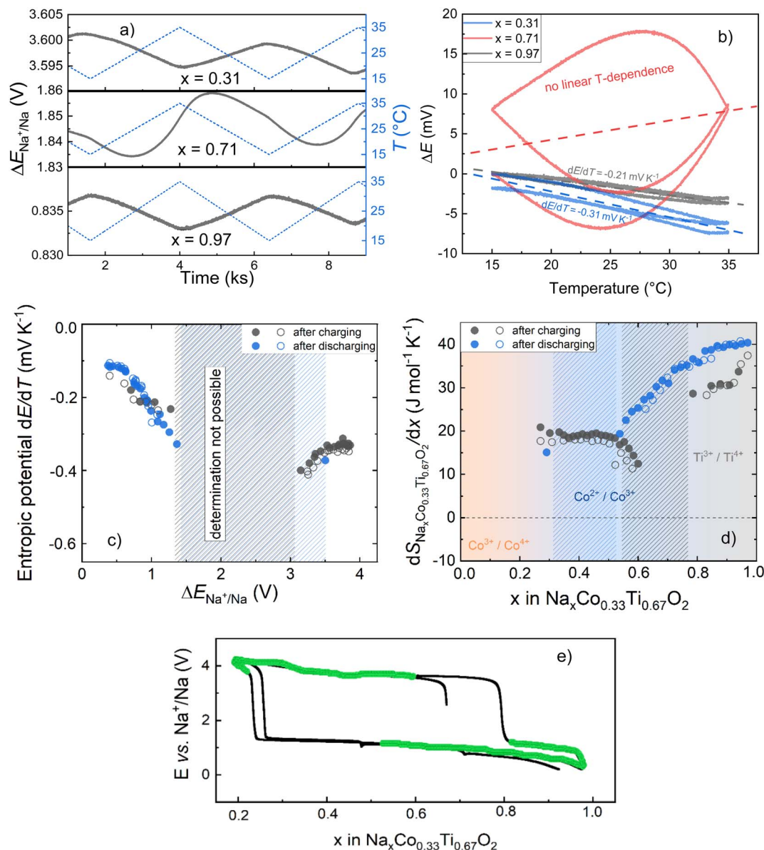
Fig. 8 (a) OCV measurement of O3- \text{Na}_x\text{Co}_{0.33}\text{Ti}_{0.67}\text{O}_2/\text{Na} half-cells at different compositions ( x = 0.31, 0.71 and 0.97 ) during linear temperature variations. (b) Temperature dependence of the OCV determined from the measured data and associated linear fits (dashed lines) to determine dE/dT and \Delta rS^0 , respectively. Note that for reasons of comparability, the initial OCV value was subtracted in each case. (c) Entropic potential of the O3- \text{Na}_x\text{Co}_{0.33}\text{Ti}_{0.67}\text{O}_2/\text{Na} half-cells plotted against OCV, and (d) the composition dependence of the partial molar entropy change of O3- \text{Na}_x\text{Co}_{0.33}\text{Ti}_{0.67}\text{O}_2 with respect to x for two identical cells. The entropic potential dE/dT was determined by temperature-dependent measurements of the equilibrium potential for each SoC, in case of a linear temperature dependence of OCV. Shaded areas indicate anomalous temperature dependence of OCV either after charging or discharging, in which reliable entropy determination was not always possible. (e) Composition-dependent charge-discharge curves of O3- \text{Na}_x\text{Co}_{0.33}\text{Ti}_{0.67}\text{O}_2 with marked composites (green color), for which entropy determination in OCV measurements was possible.
