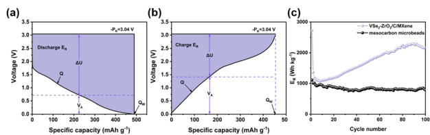
Fig. 5 Typical legends for the determination of the relative energy density ( E_R ) of (a) discharge E_R and (b) charge E_R . (c) Discharge E_R of \text{VSe}_2\text{-ZrO}_2\text{/C/MXene} and meso-carbon microbeads.
