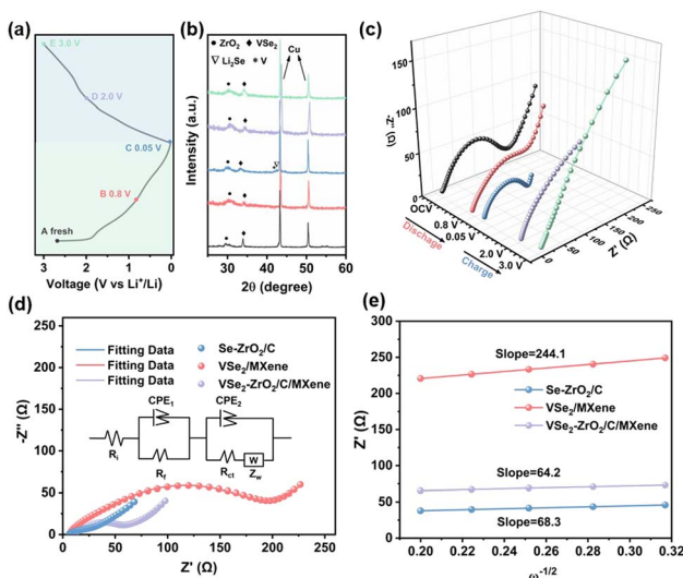
Fig. 6 (a) Discharge/charge curve and corresponding voltage positions of \text{VSe}_2\text{-ZrO}_2\text{/C/MXene} . (b) Ex situ XRD characterizations of the corresponding potential states. (c) EIS plots of \text{VSe}_2\text{-ZrO}_2\text{/C/MXene} at various states in the 40th cycle at 100 \text{mA g}^{-1} . (d) Nyquist plots of \text{Se-ZrO}_2\text{/C} , \text{VSe}_2\text{/MXene} and \text{VSe}_2\text{-ZrO}_2\text{/C/MXene} after 100 cycles at 100 \text{mA g}^{-1} (inset: corresponding equivalent circuit model). (e) Fitted lines of Z' versus \omega^{-1/2} at low frequency for \text{VSe}_2\text{-ZrO}_2\text{/C/MXene} .
